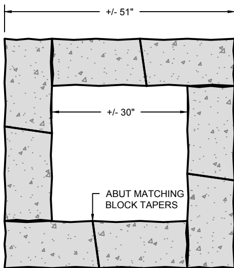
BOTTOM COURSE (PLAN VIEW)
