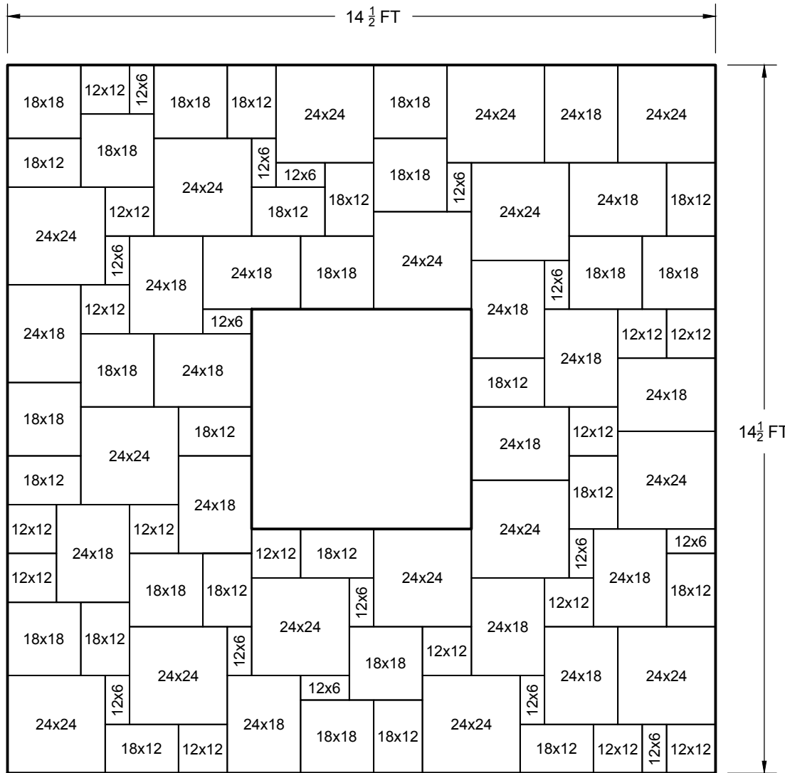
DIMENSIONAL FLAGSTONE PATIO DIMENSIONS & LAYOUT (PLAN VIEW)
