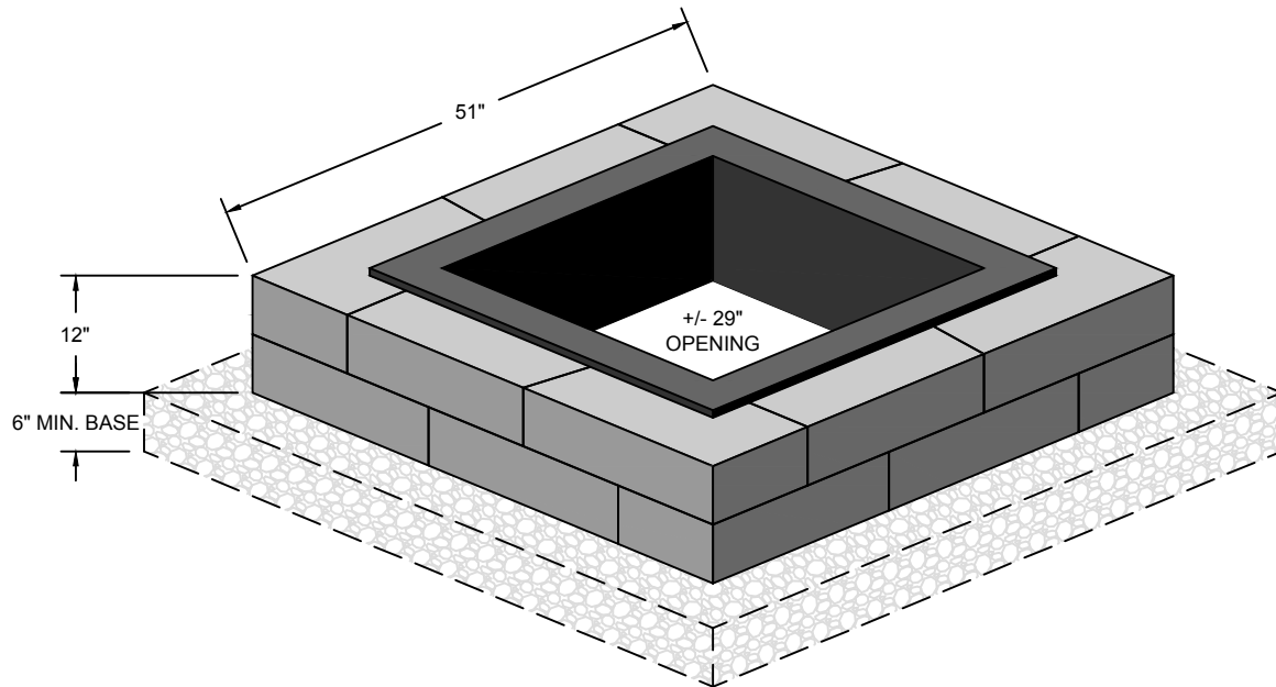
TYPICAL CONSTRUCTION (ISOMETRIC VIEW)
